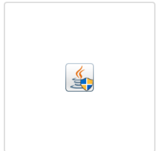
jdk-8u171-windows-x64.exe
